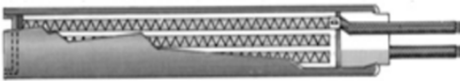
Figure 1: A standard cartridge heater. Source: Backer Hotwatt Inc.
