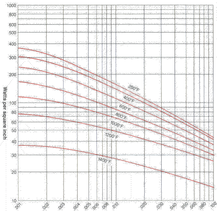
Figure 3: Maximum watt density for Superwatt swaged cartridge heaters with various increasing temperatures and hole tolerances. Source: Backer Hotwatt
