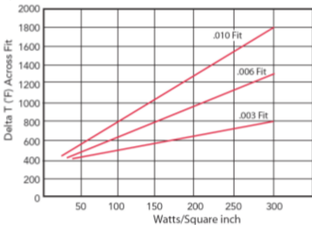
Figure 6: Temperature differential across fit as a function of watt density. Source: Backer Hotwatt
