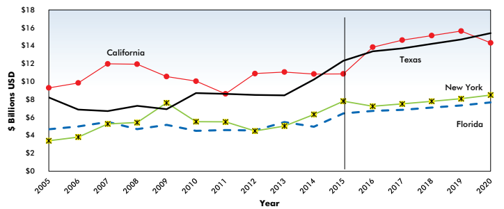
Graph 18: U.S. Four Largest States: Total Engineering/Civil Construction Starts – CMD
