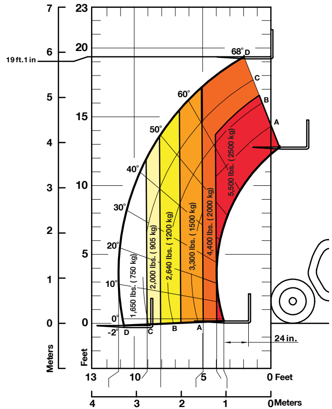
Load Chart based on 24 inch (600 mm) load center per B56.6.
